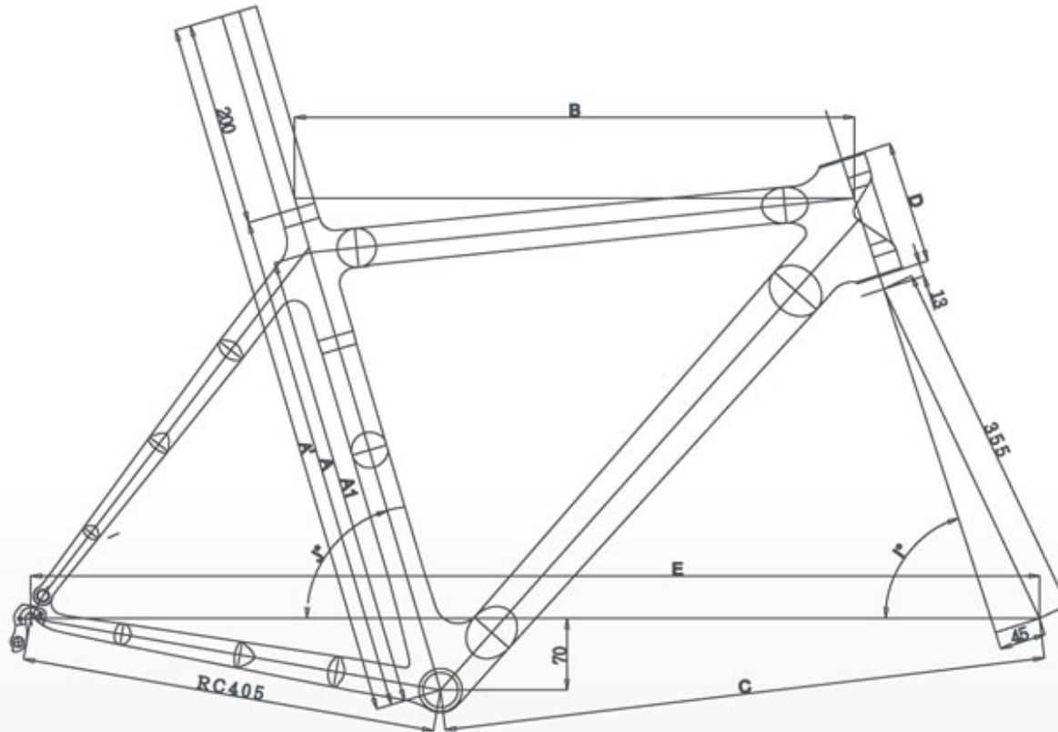
RQC / RLC Frame Geometry
