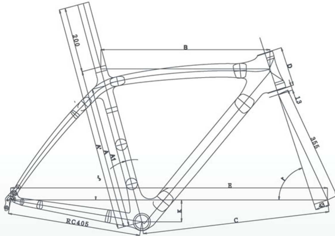
RQC Frame Geometry
