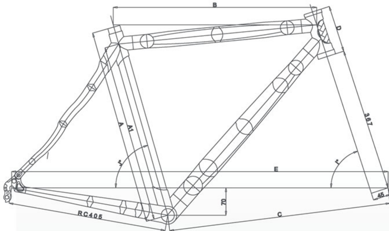
RCC / RAC Frame Geometry
