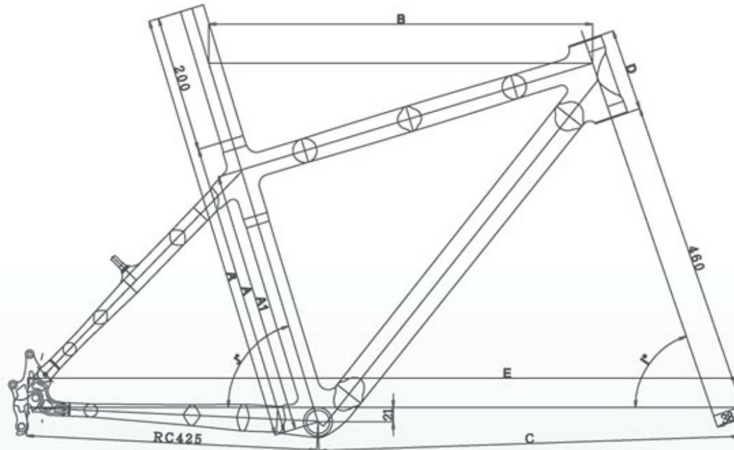
MQC Frame Geometry
