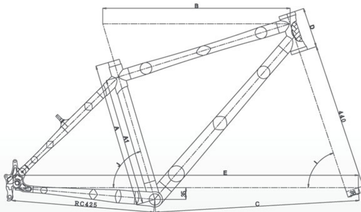
MCC / MAC Frame Geometry
